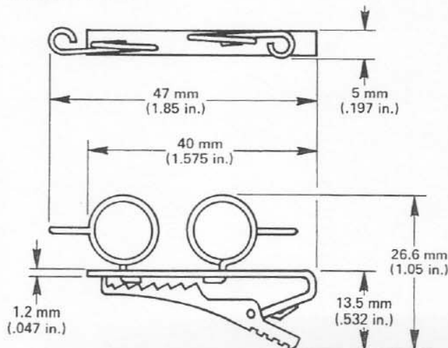
FIGURE 1 — 390/390A Dimensions
